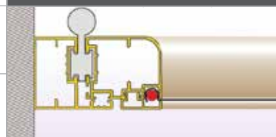
ΠΡΟΦΙΛ "L" STANDARD FRAME PROFILE "L" STANDARD
